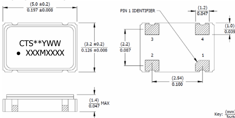
PACKAGE DRAWING
