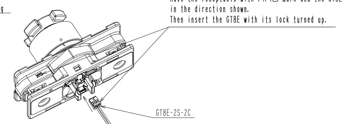
3 View of signal contact side
