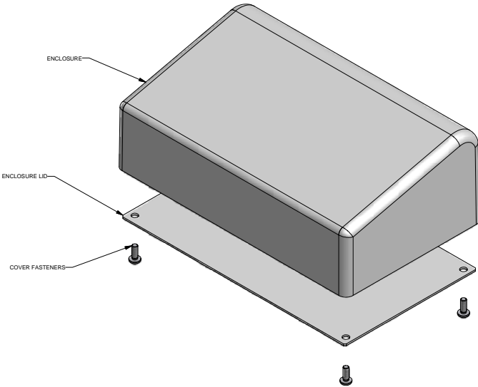
ENCLOSURE ASSEMBLY
