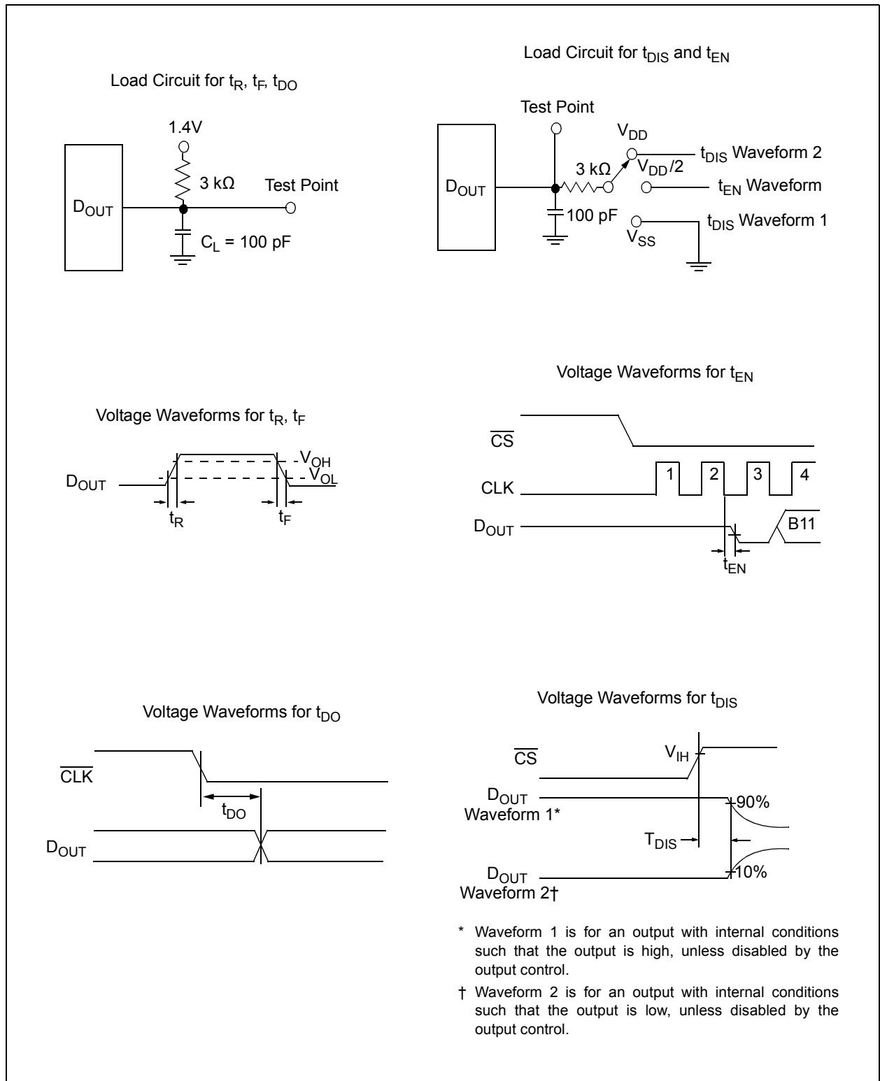
FIGURE 1-2: Test Circuits.
