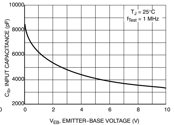
Figure 16. Input Capacitance
