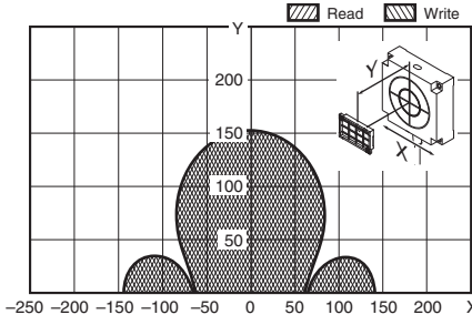
V680-HS65 (with Metal on Back Surface) & V680S-DKF68 (Tag direction: Horizontal)
