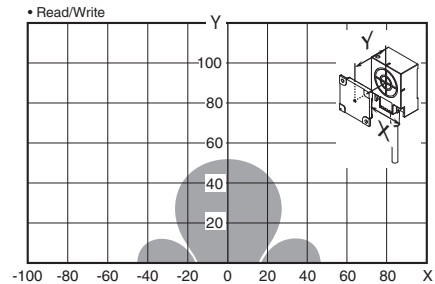
V680-HS63 (mounted on non-metallic material) & V680S-D8KF67
