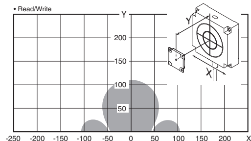
V680-HS52 (embedded on non-metallic material) & V680S-D8KF67M (mounted on metallic surface: steel)
