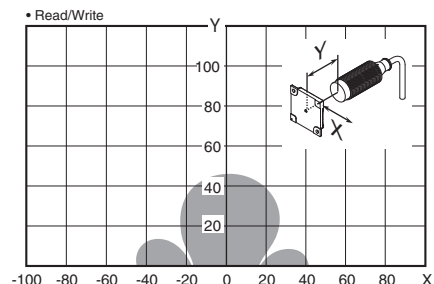
V680-HS65 (mounted on metallic material) & V680S-D8KF67
