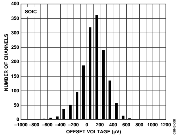
Figure 11. Input Offset Voltage Distribution, V SY = ±15 V
