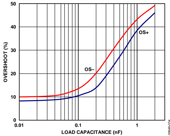
Figure 39. Overshoot vs. Load Capacitance, V_{SY} = \pm 5 V , A_V = +1 , R_L = 2 k\Omega , V_{IN} = 100 mV p-p
