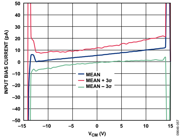
Figure 17. Input Bias Current vs. Common-Mode Input Voltage ( V_{CM} ), V_{SY} = \pm 15 V, R_L = \infty
