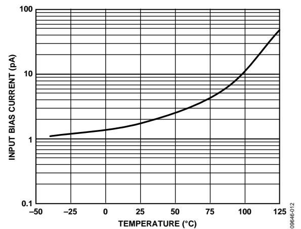
Figure 19. Input Bias Current vs. Temperature, V_{SY} = \pm 15 V
