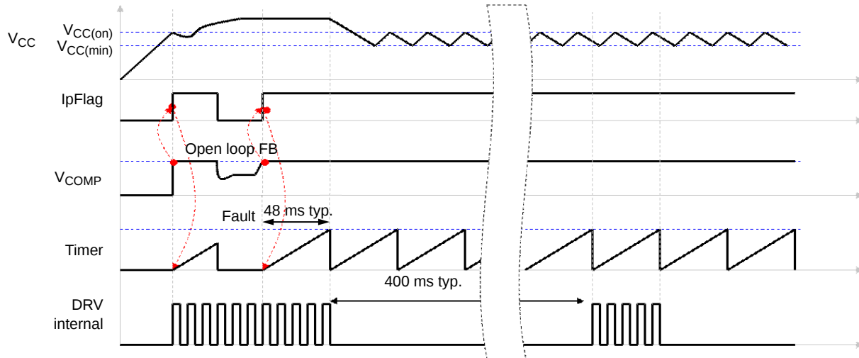
Figure 31. In case of short-circuit or overload, the NCP106X protects itself and the power supply via a low frequency burst mode. The V_{CC} is maintained by the current source and self-supplies the controller.
