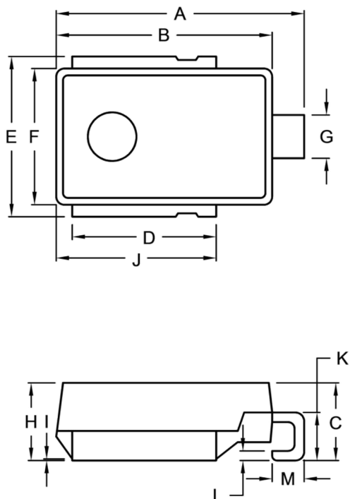
DO-218AB
