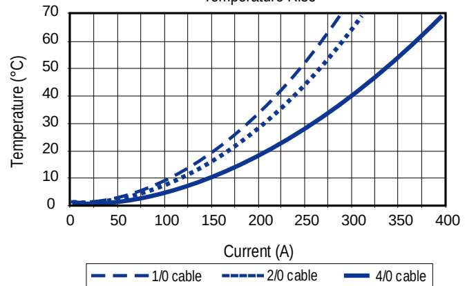
PowerMod®HP Dual Pole Series “B” Temperature Rise
