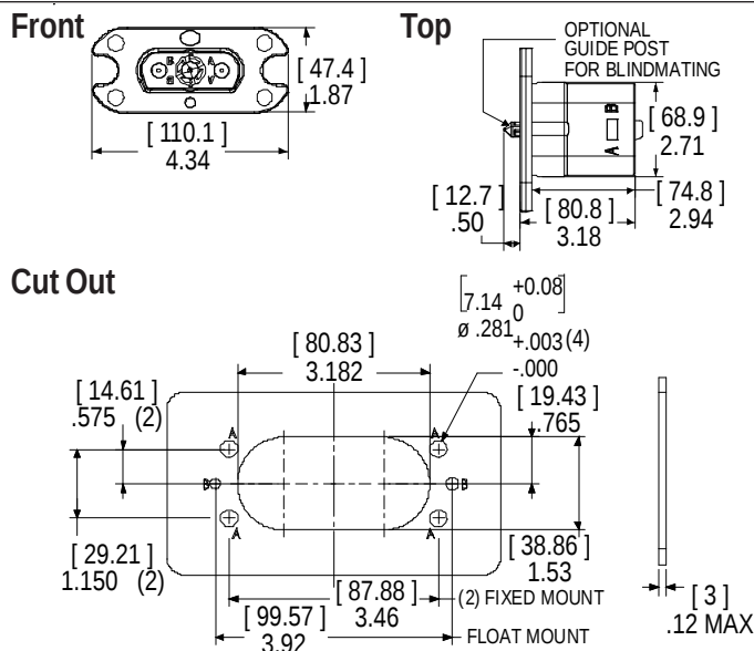
Dual Pole Straight Female
