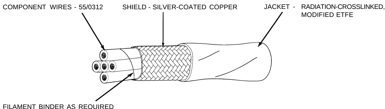
CABLE CONSTRUCTION DETAILS
