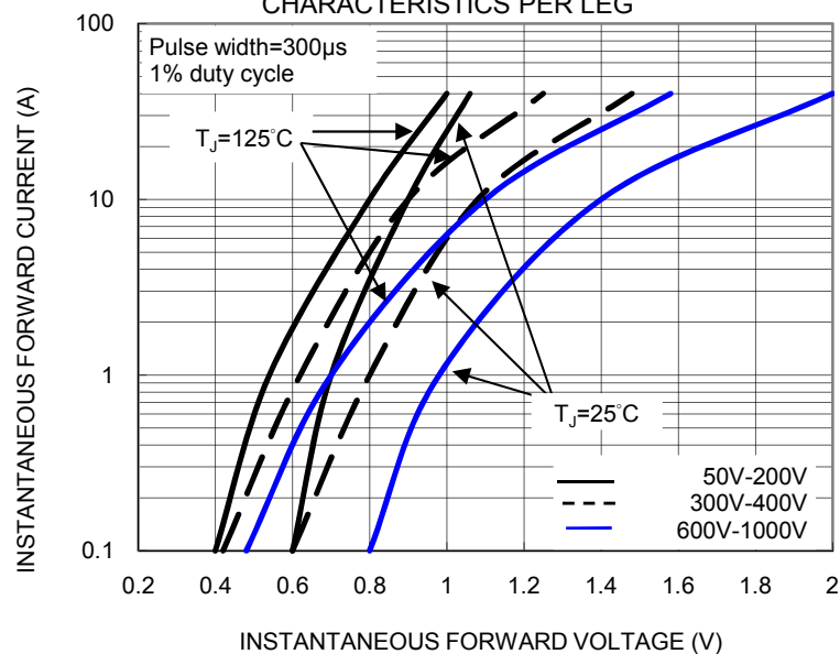
FIG. 4 TYPICAL INSTANTANEOUS FORWARD CHARACTERISTICS PER LEG
