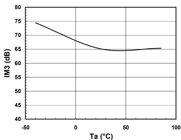
IM3 vs. Ta
