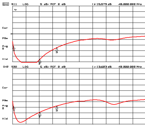
S11, S22 (f=10MHz to 3GHz)
