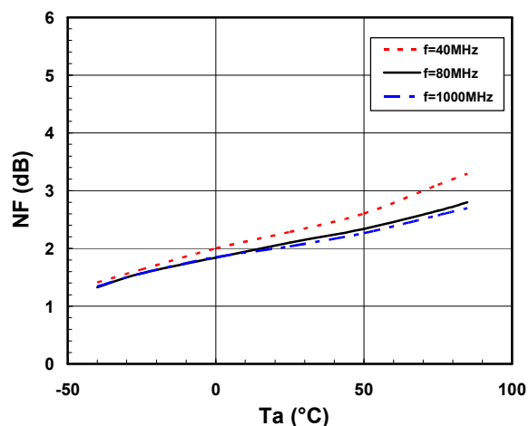
NF vs. Ta
