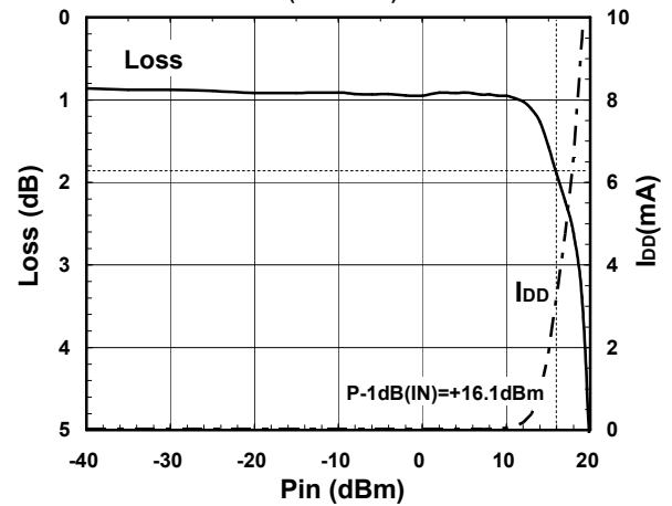
Loss, I_{DD} vs. P_{in}
