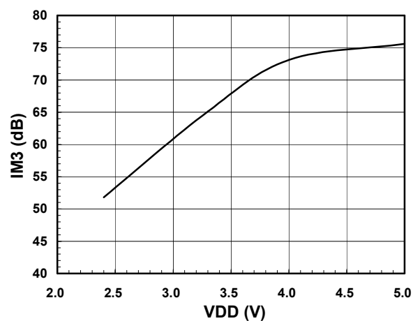
IM3 vs. VDD
