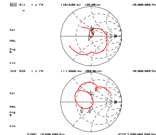
Z in , Z out (f=10MHz to 3GHz)
