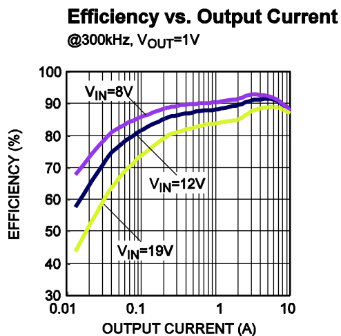
Figure 18 — Efficiency Curve
