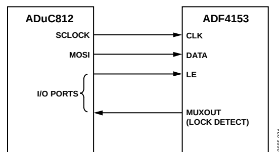
Figure 18. ADuC812 to ADF4153 Interface
