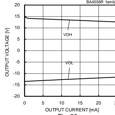
Fig. 30 Maximum Output Voltage - Output Current
