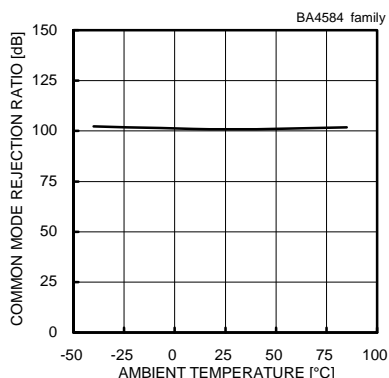
Fig. 148 Common Mode Rejection Ratio - Ambient Temperature (VCC/VEE=±15[V]/-15[V], Vicm=-12[V] to +12[V])
