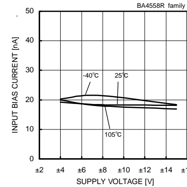
Fig. 33 Input Bias Current - Supply Voltage
