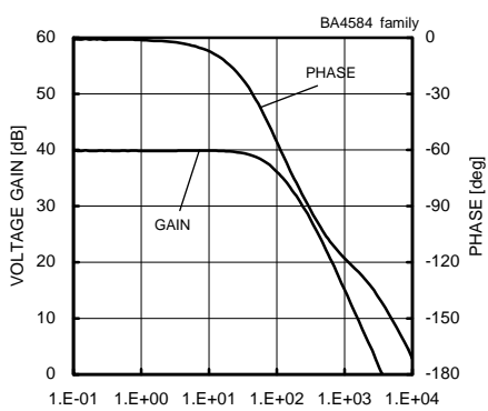
Fig. 154 Voltage Gain - Frequency (VCC/VEE=±15[V]/-15[V], Av=40[dB], RL=2[kΩ], Ta=25[°C])
