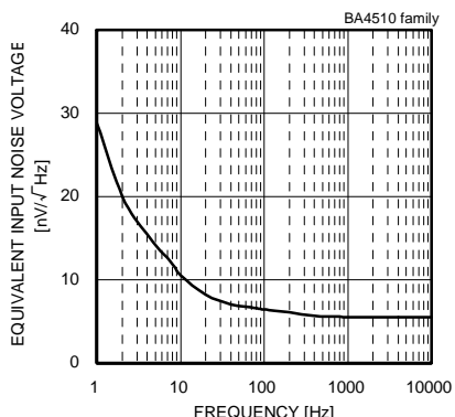
Fig. 286 Equivalent Input Noise Voltage - Frequency (V CC /V EE =2.5[V]/-2.5[V])
