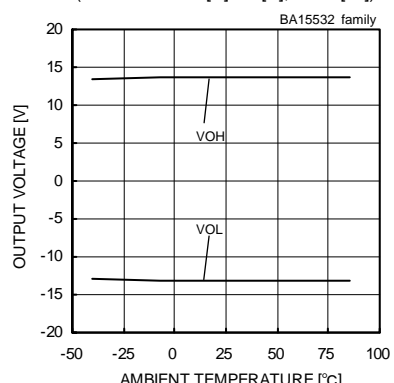
Fig. 249 Maximum Output Voltage - Ambient Temperature (VCC/VEE=+15[V]/-15[V], RL=2[kΩ])
