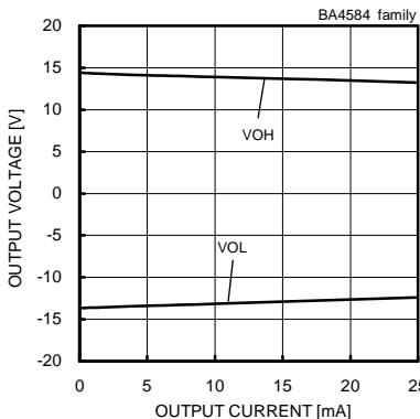
Fig. 140 Maximum Output Voltage - Output Current (VCC/VEE=+15[V]/-15[V], Ta=25[°C])
