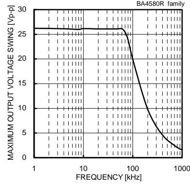
Fig. 131 Maximum Output Voltage Swing - Frequency ( V_{CC}/V_{EE}=+15[V]/-15[V] , R_L=2[kΩ] , T_a=25[°C] )
