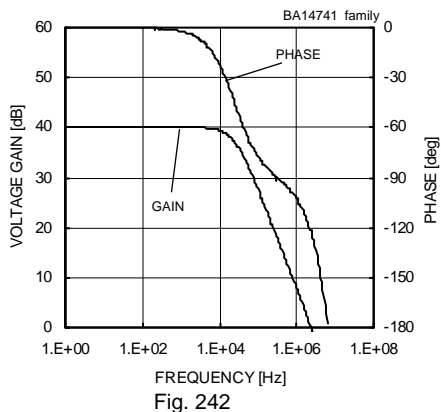
Fig. 242 Voltage Gain - Frequency ( V_{CC}/V_{EE}=+15[V]/-15[V] , A_v=40[dB] , R_L=2[k\Omega] , T_a=25[^\circ C] )
