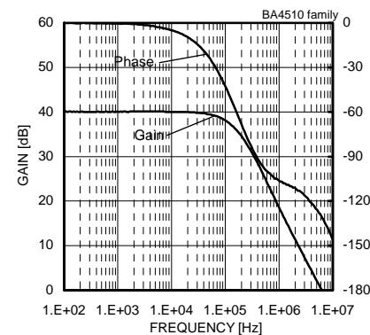
Fig. 287 Voltage Gain - Frequency ( V_{CC}/V_{EE}=2.5[V]/-2.5[V] , A_v=40[dB] , R_L=10[k\Omega] )
