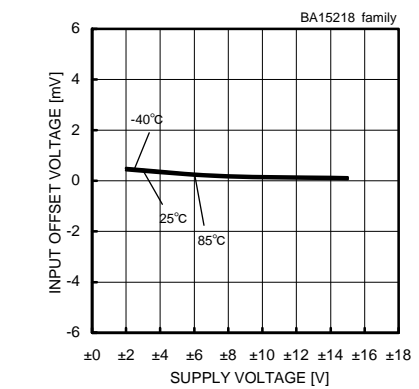
Input Offset Voltage - Supply Voltage (Vicm=0[V], Vout=0[V])
