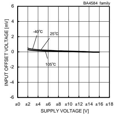
Fig. 141 Input Offset Voltage - Supply Voltage (Vicm=0[V], Vout=0[V])
