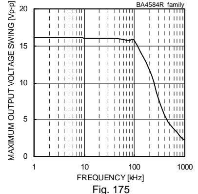
Fig. 175 Maximum Output Voltage Swing - Frequency ( V_{CC}/V_{EE}=+9.5[V]/-9.5[V] , R_L=2[k\Omega] , T_a=25[^\circ C] )
