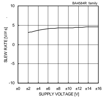
Fig. 172 Slew Rate - Supply Voltage ( C_L=100[pF] , R_L=2[k\Omega] , T_a=25[^\circ C] )
