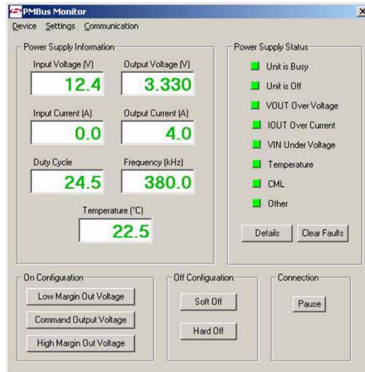
Figure 5. View of the PMBus Monitor
