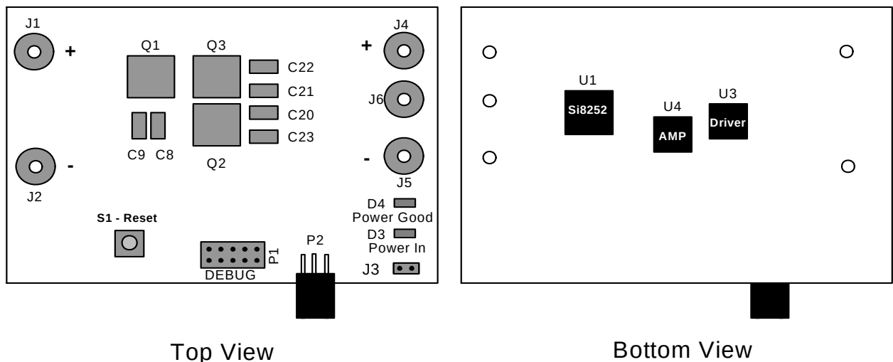
Figure 15. Si8252 Single-Phase POL Target Board
