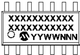
14-Lead SOIC (3.90 mm) ( MCP6474 only )
