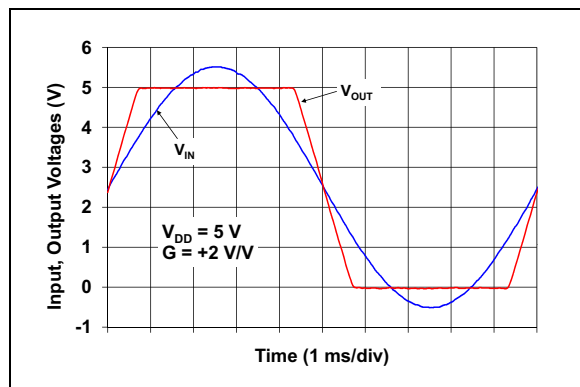
FIGURE 2-32: The MCP6471/2/4 Shows No Phase Reversal.
