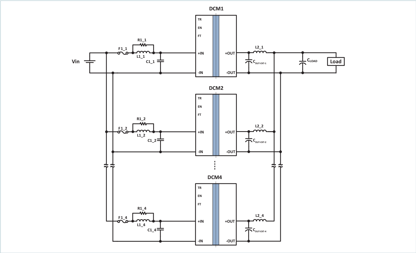
Typical Application 1: DCM4623xD2K26E0yzz in an array of four units
