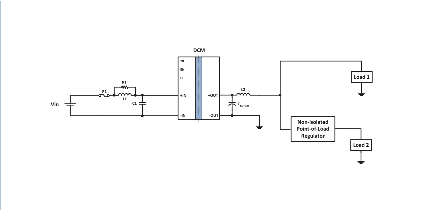
Typical Application 2: Single DCM4623xD2K26E0yzz, to a non-isolated regulator, and direct to load
