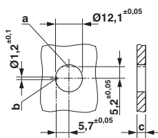
Dimensional drawing
