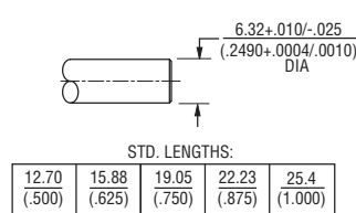
SHAFT TYPE "A" (USES BUSHING A)
