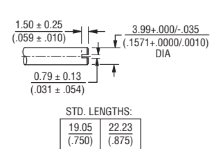
SHAFT TYPE "V" (USES BUSHING U)
