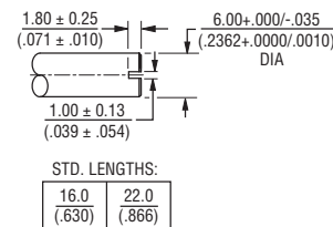
SHAFT TYPE "J" (USES BUSHING R)
