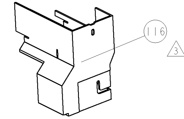
AMP-O-LECTRIC TERM GUARD
