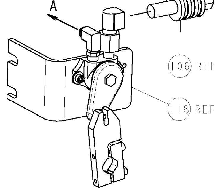
AIR FEED VALVE ASM (-2 ONLY)
