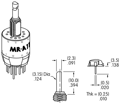
Shaft Terminal
