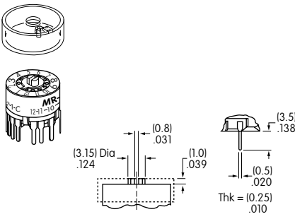
Slotted for Screwdriver Terminal
