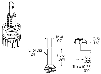
Shaft Terminal
