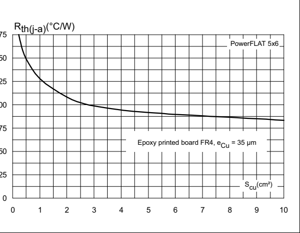
Figure 8. Thermal resistance, junction to ambient, versus copper surface under tab (typical values)
