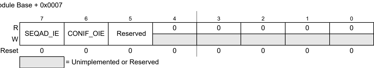
Figure 9-11. ADC Interrupt Enable Register (ADCIE)
