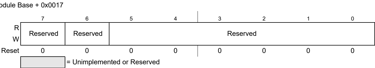
Figure 9-21. ADC Command Register 3 (ADCCMD_3)
