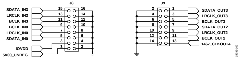
Figure 101. Serial Port Header Schematic
