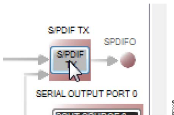
Figure 45. Configuring the S/PDIF Transmitter Routing Matrix Register
