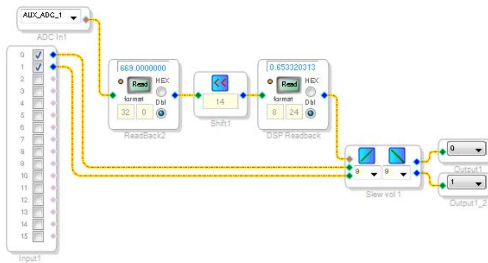
Figure 62. Completed Signal Flow with DSP Readback
