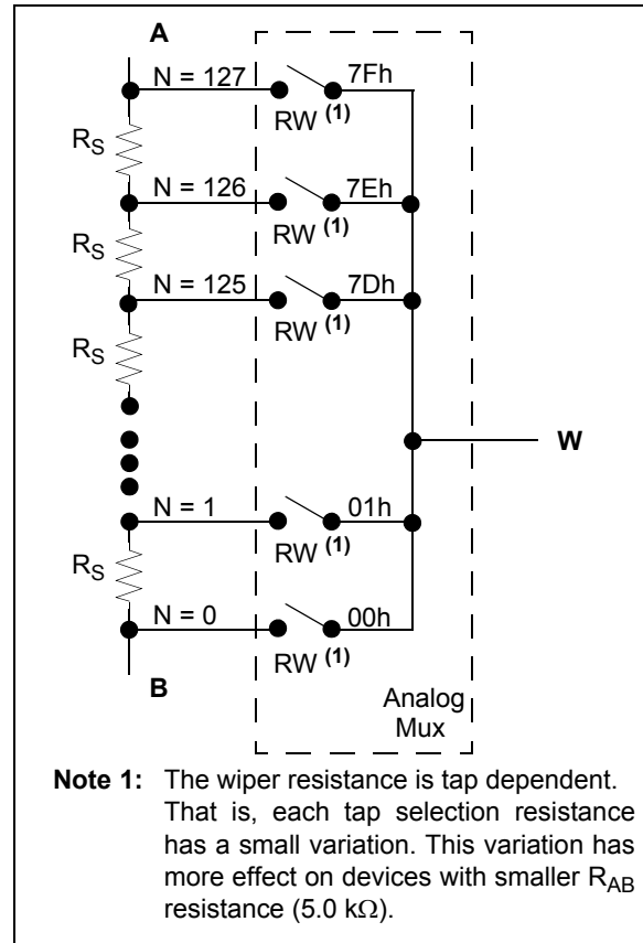
FIGURE 6-1: Resistor Network Block Diagram.
