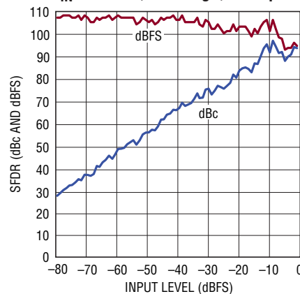
LTC2263-14: SFDR vs Input Level, f_{IN} = 70\text{MHz} , 2V Range, 25MSPS
