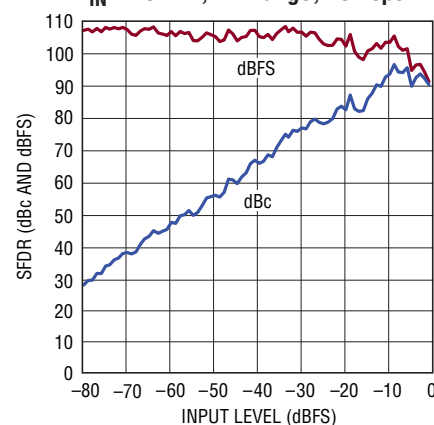
LTC2264-14: SFDR vs Input Level, f_{IN} = 70\text{MHz} , 2V Range, 40Msps
