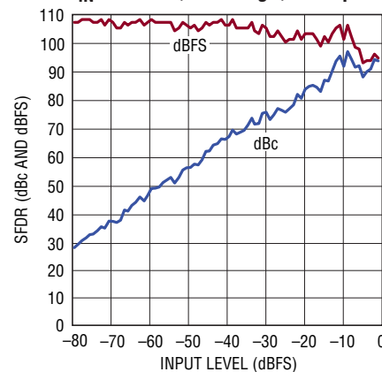
LTC2263-14: SFDR vs Input Level, f_{IN} = 70\text{MHz} , 2V Range, 25Mps
