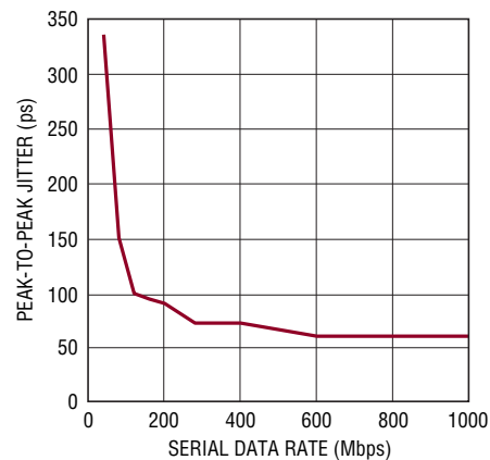
DCO Cycle-Cycle Jitter vs Serial Data Rate
