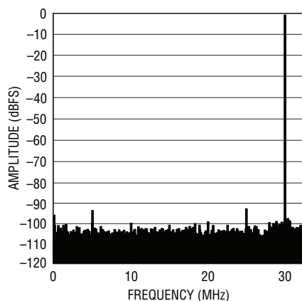
LTC2265-14: 8k Point FFT, f_{IN} = 30\text{MHz} , -1\text{dBFS} , 65Mps
