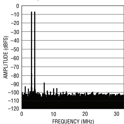
LTC2265-14: 8k Point 2-Tone FFT, f_{IN} = 68\text{MHz} , 69MHz, -1\text{dBFS} , 65Mps
