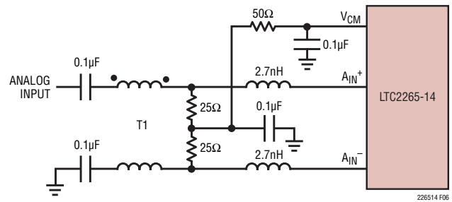
Figure 6. Recommended Front-End Circuit for Input Frequencies Above 300MHz
