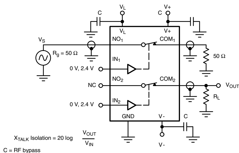
Fig. 5 - Crosstalk
