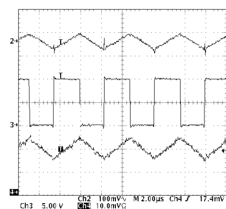
PWM Operation 5 V Converter ( V_{IN} = 10\text{ V} )
