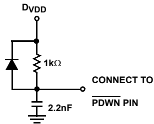
FIGURE 36. PDWNDELAY CIRCUIT
