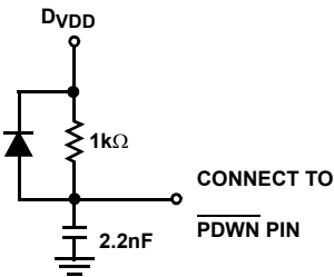
FIGURE 36. PDWNDELAY CIRCUIT
