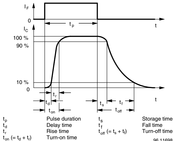
Fig. 2 - Switching Times
