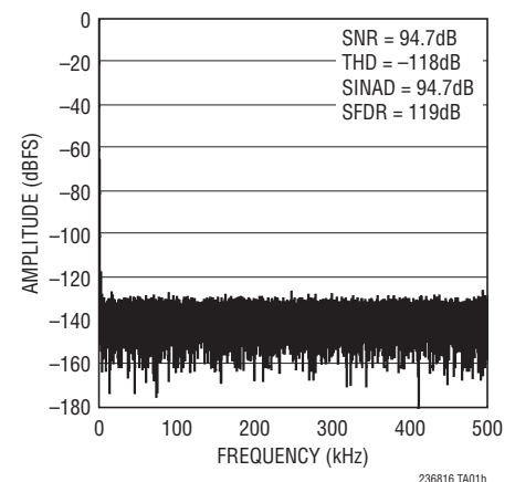
32k Point FFT f_{\text{S}} = 1\text{Mps} , f_{\text{IN}} = 2\text{kHz}
