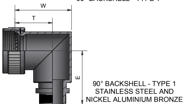
90° BACKSHELL - TYPE 1
