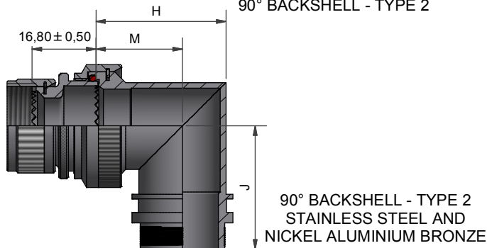
90° BACKSHELL - TYPE 2
