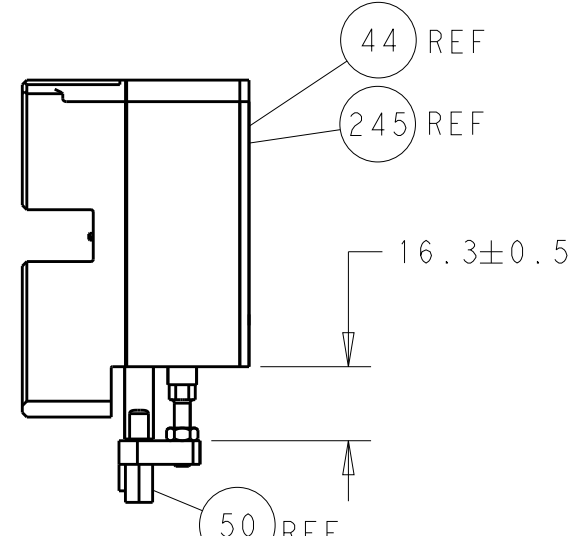
HOLDDOWN SET-UP
